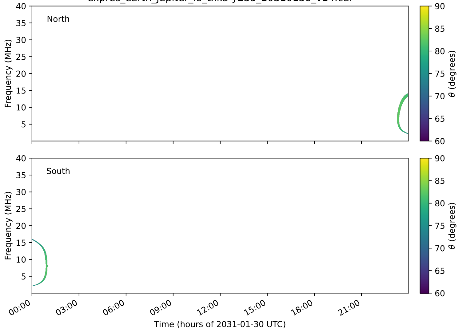
expres_earth_jupiter_io_txka-y235_20310130_v14.cdf
