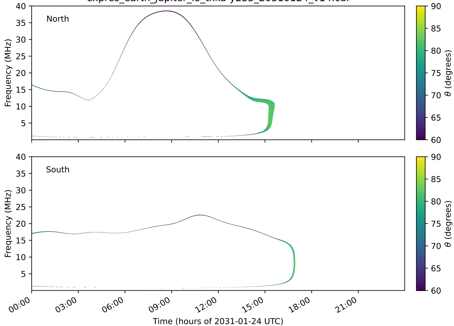
expres_earth_jupiter_io_txka-y235_20310124_v14.cdf
