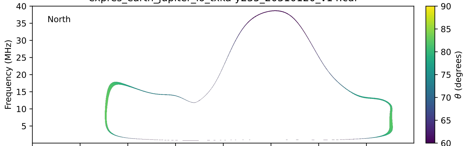
expres_earth_jupiter_io_txka-y235_20310120_v14.cdf
