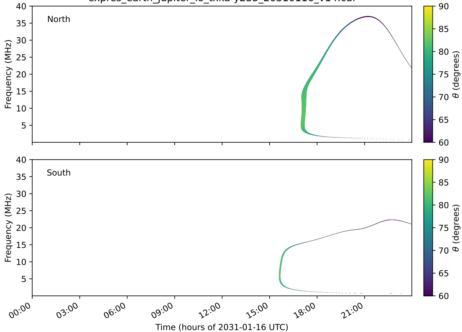
expres_earth_jupiter_io_txka-y235_20310116_v14.cdf
