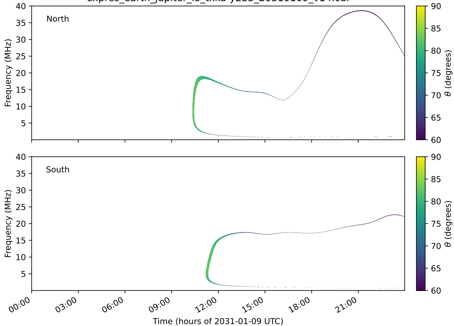
expres_earth_jupiter_io_txka-y235_20310109_v14.cdf
