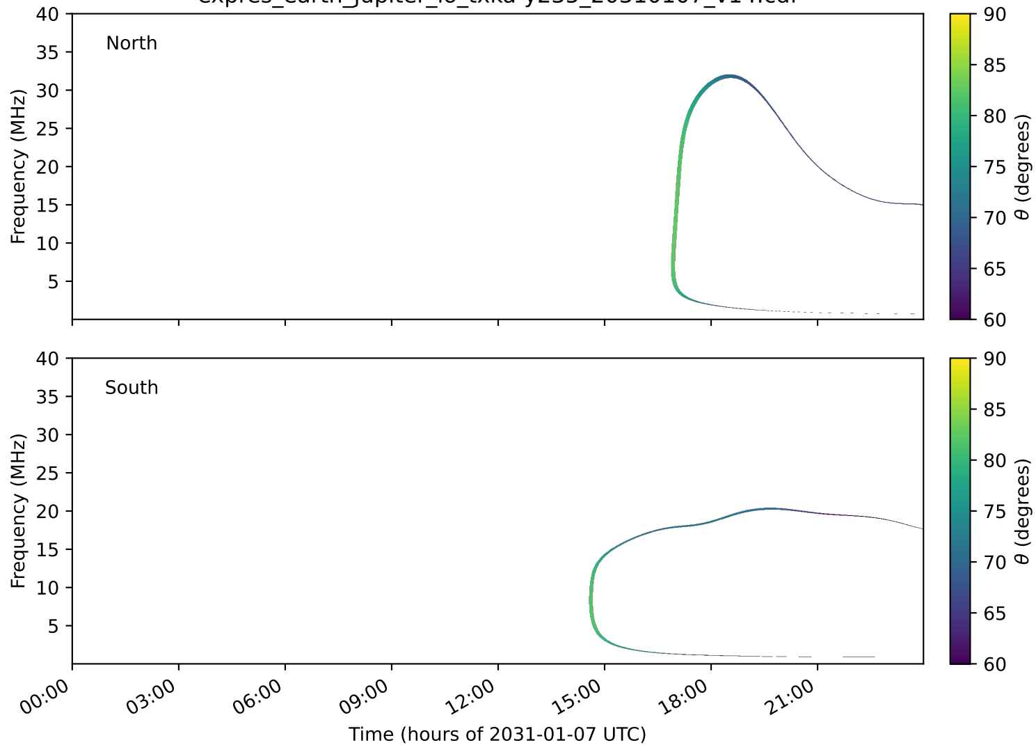
expres_earth_jupiter_io_txka-y235_20310107_v14.cdf
