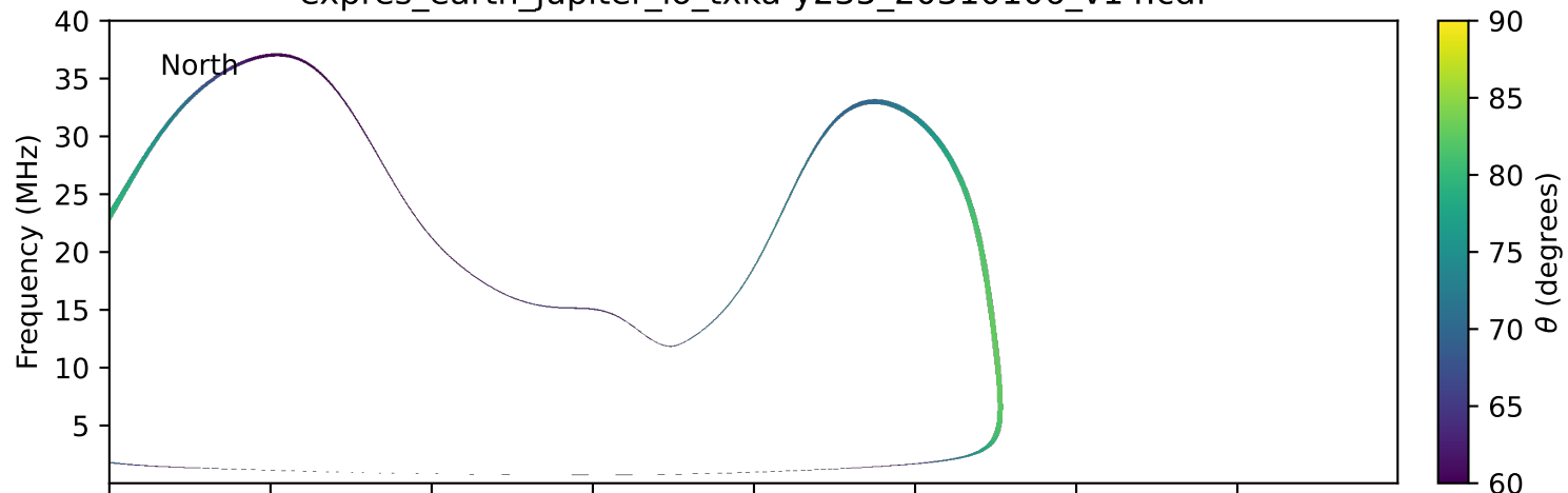
expres_earth_jupiter_io_txka-y235_20310106_v14.cdf
