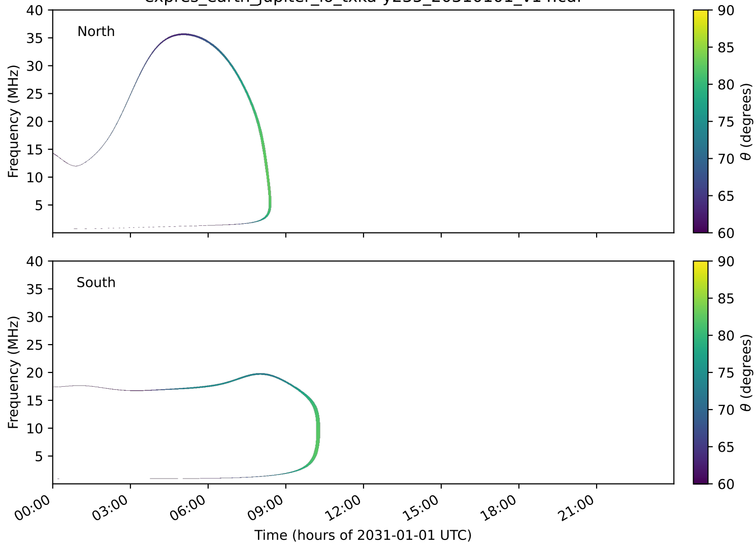
expres_earth_jupiter_io_txka-y235_20310101_v14.cdf
