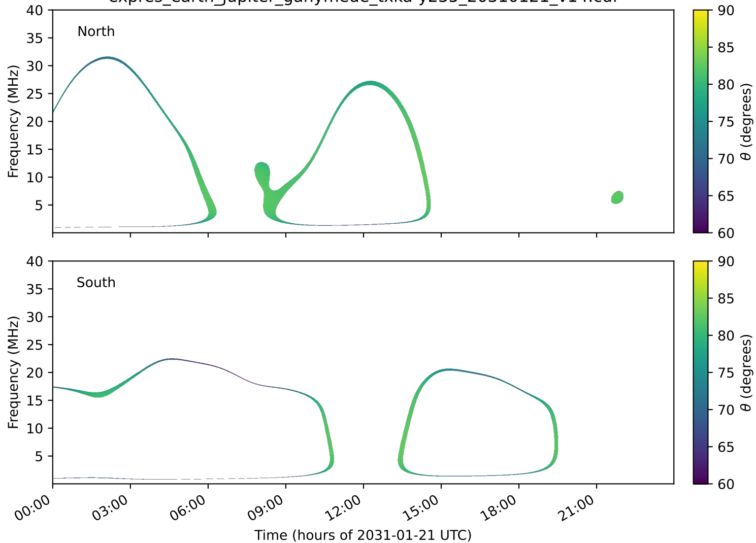
expres_earth_jupiter_ganymede_txka-y235_20310121_v14.cdf
