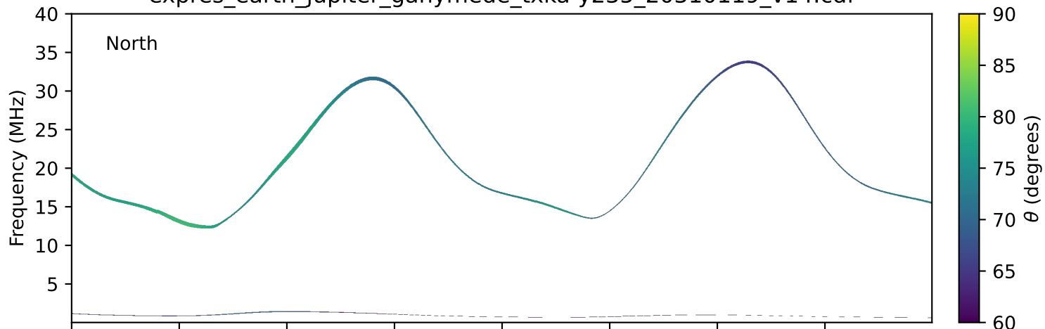
expres_earth_jupiter_ganymede_txka-y235_20310119_v14.cdf
