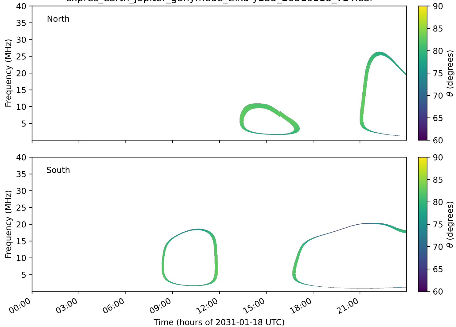
expres_earth_jupiter_ganymede_txka-y235_20310118_v14.cdf
