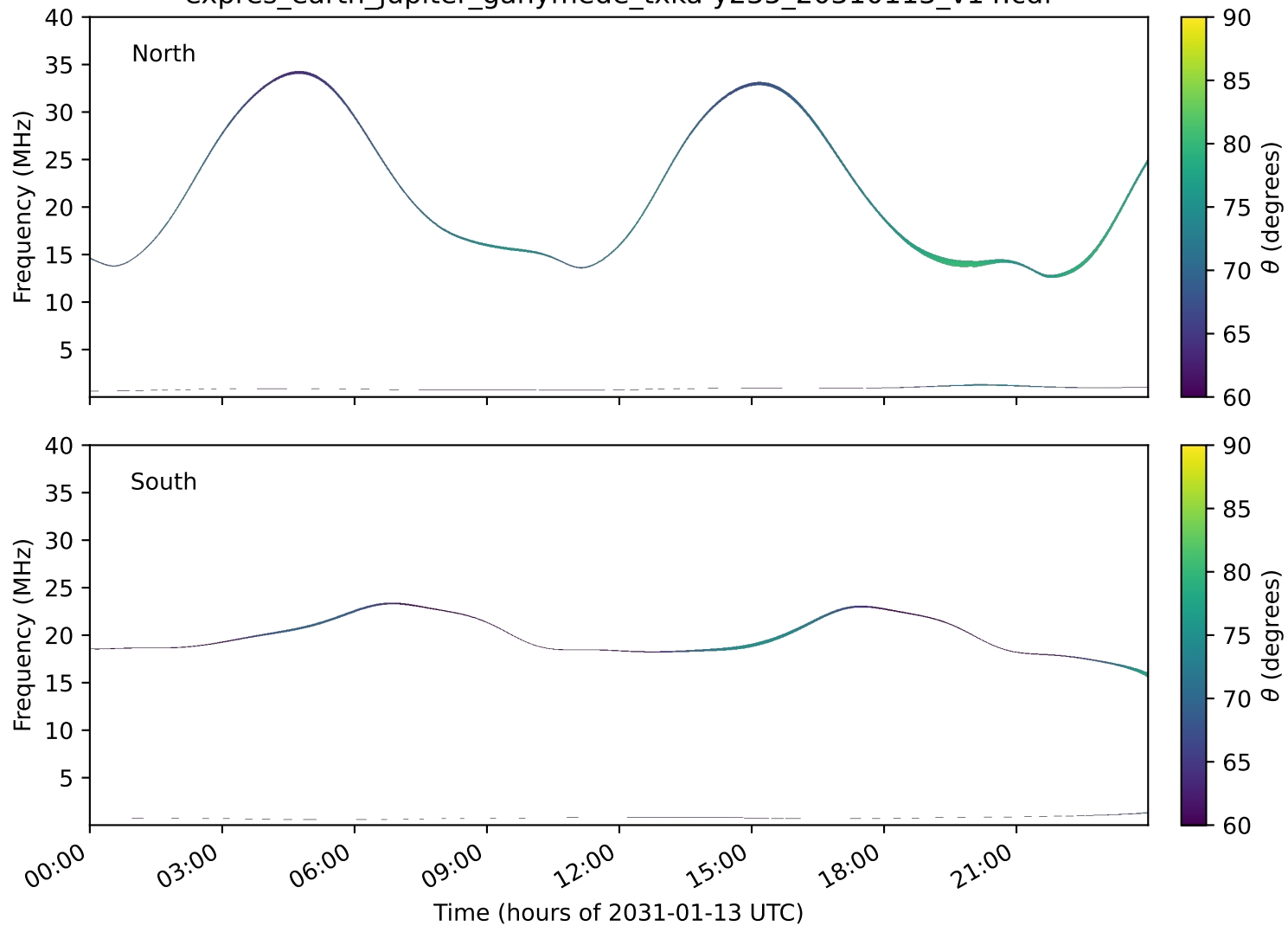
expres_earth_jupiter_ganymede_txka-y235_20310113_v14.cdf
