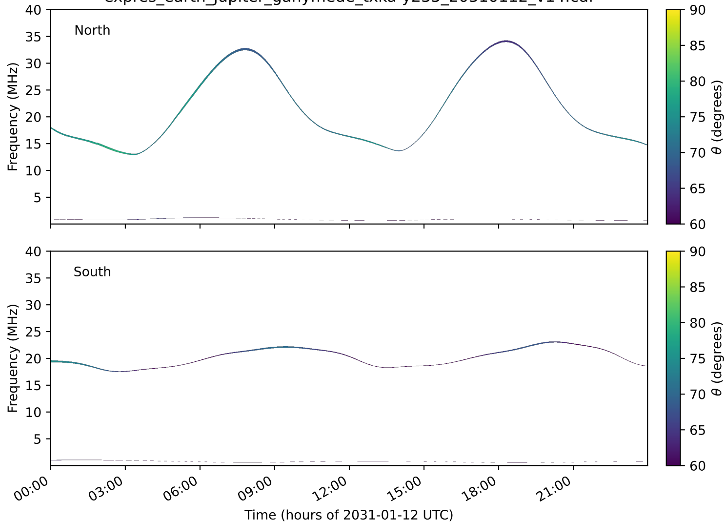
expres_earth_jupiter_ganymede_txka-y235_20310112_v14.cdf
