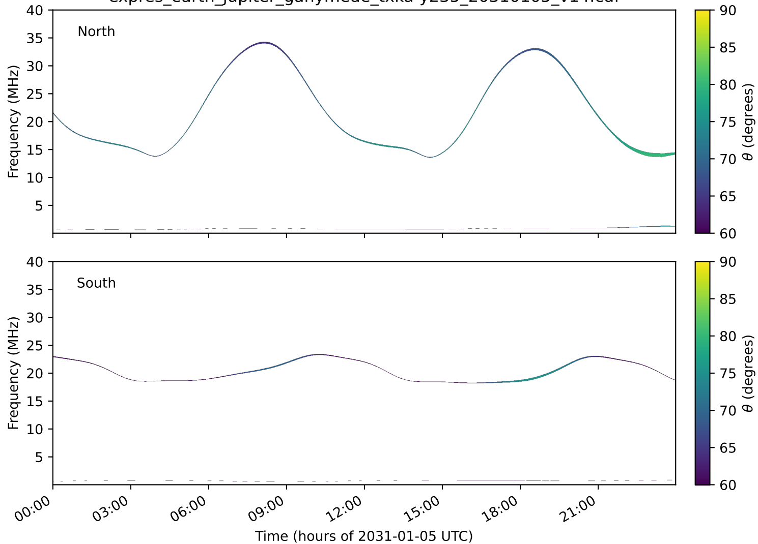
expres_earth_jupiter_ganymede_txka-y235_20310105_v14.cdf
