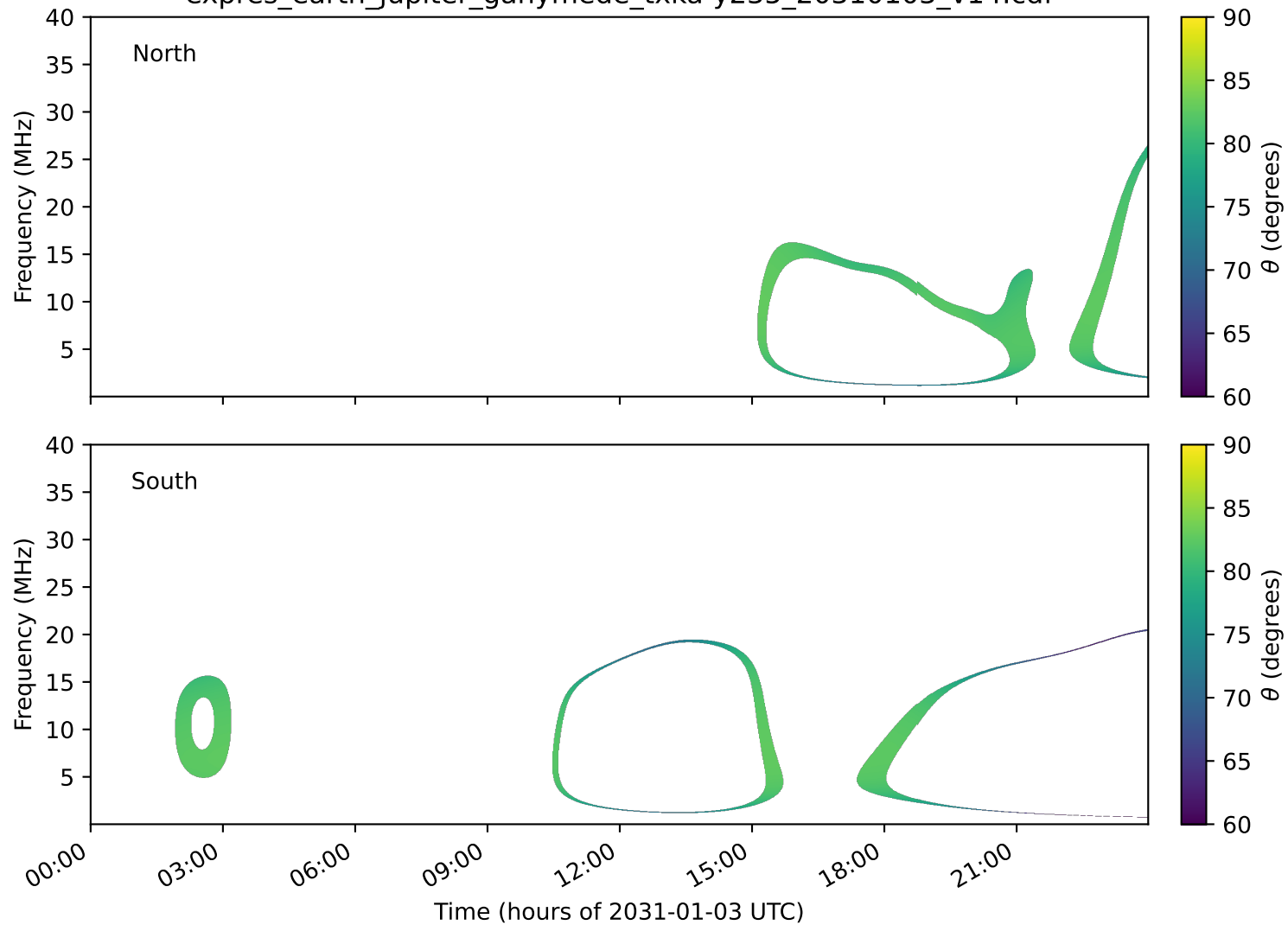
expres_earth_jupiter_ganymede_txka-y235_20310103_v14.cdf
