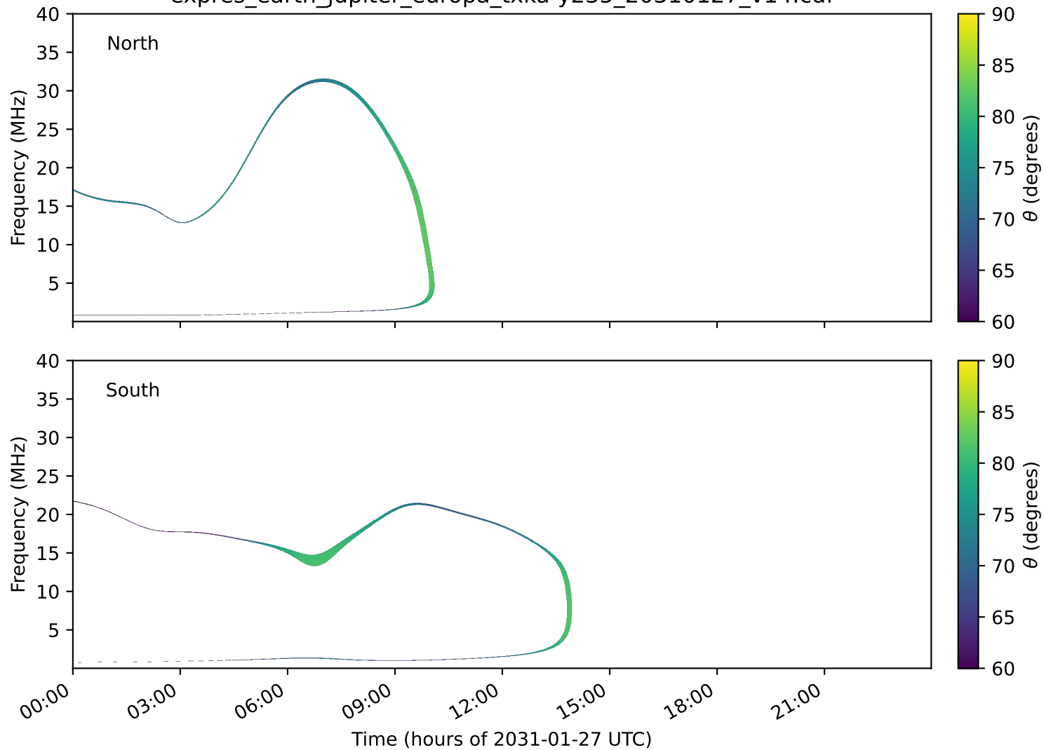
expres_earth_jupiter_europa_txka-y235_20310127_v14.cdf
