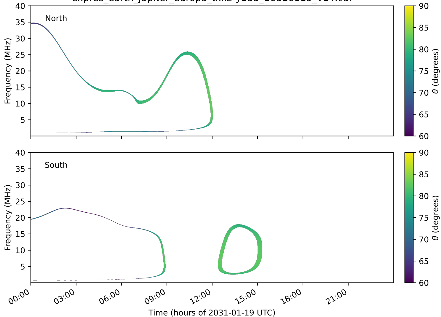
expres_earth_jupiter_europa_txka-y235_20310119_v14.cdf
