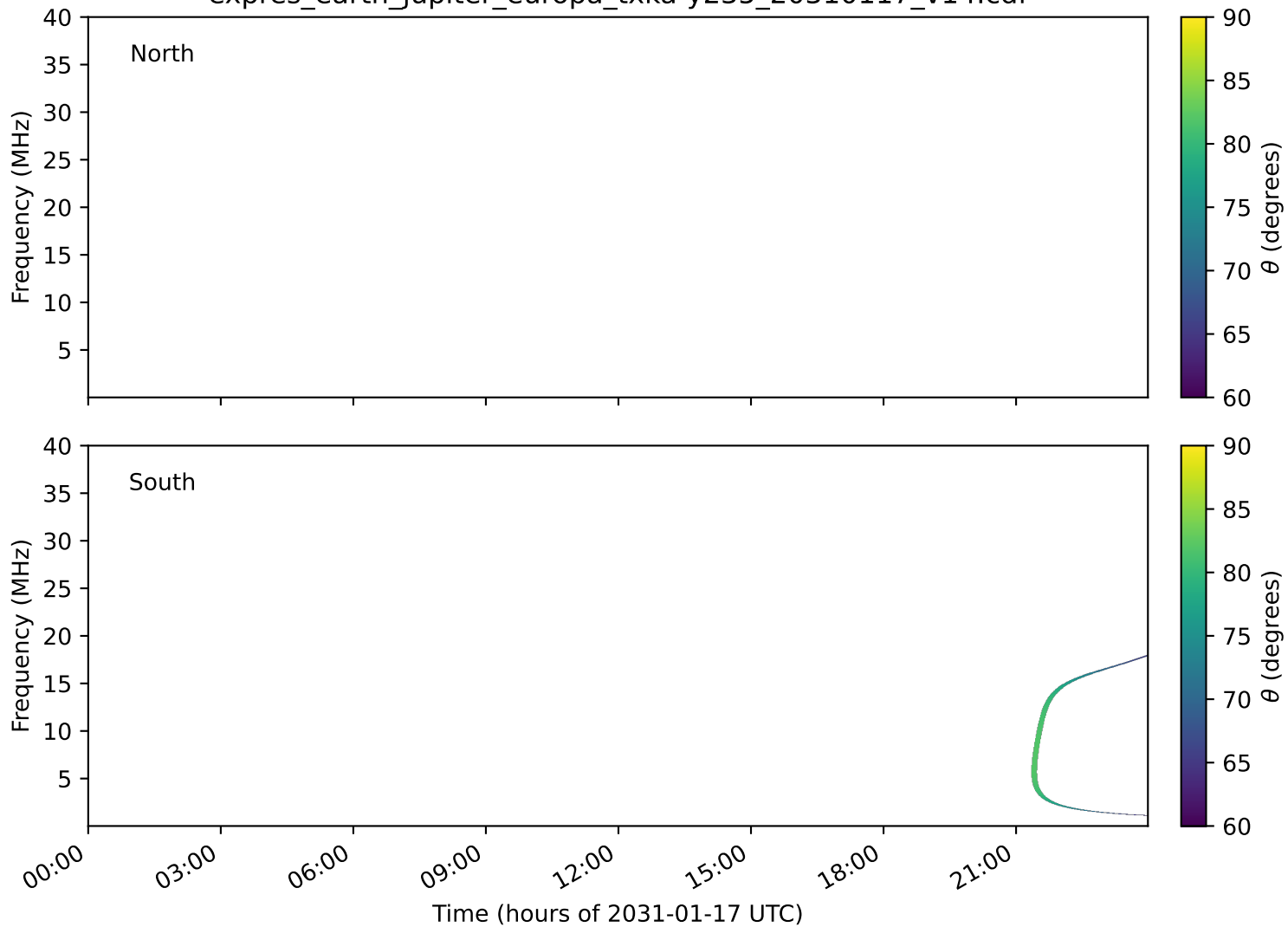
expres_earth_jupiter_europa_txka-y235_20310117_v14.cdf
