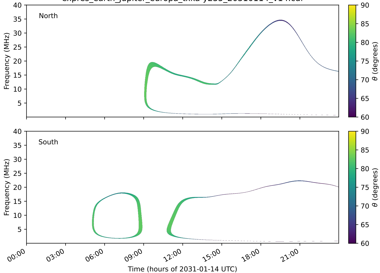
expres_earth_jupiter_europa_txka-y235_20310114_v14.cdf
