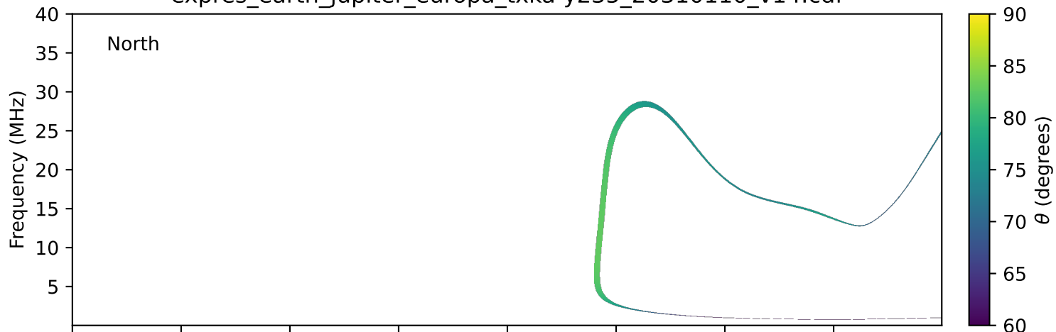
expres_earth_jupiter_europa_txka-y235_20310110_v14.cdf
