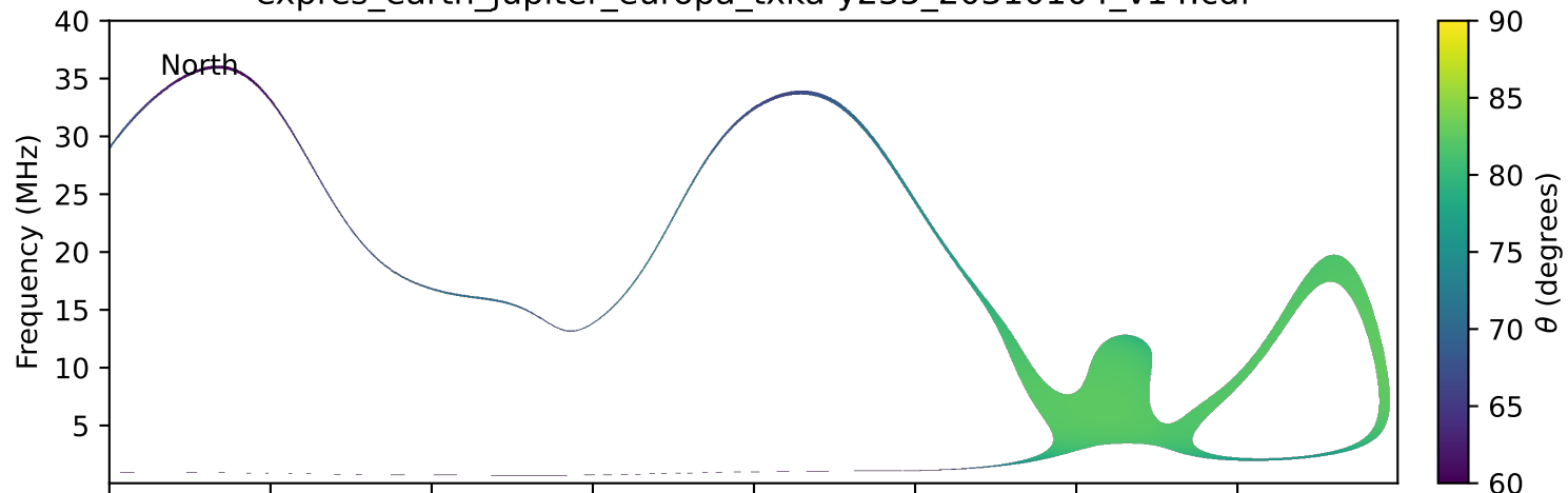
expres_earth_jupiter_europa_txka-y235_20310104_v14.cdf
