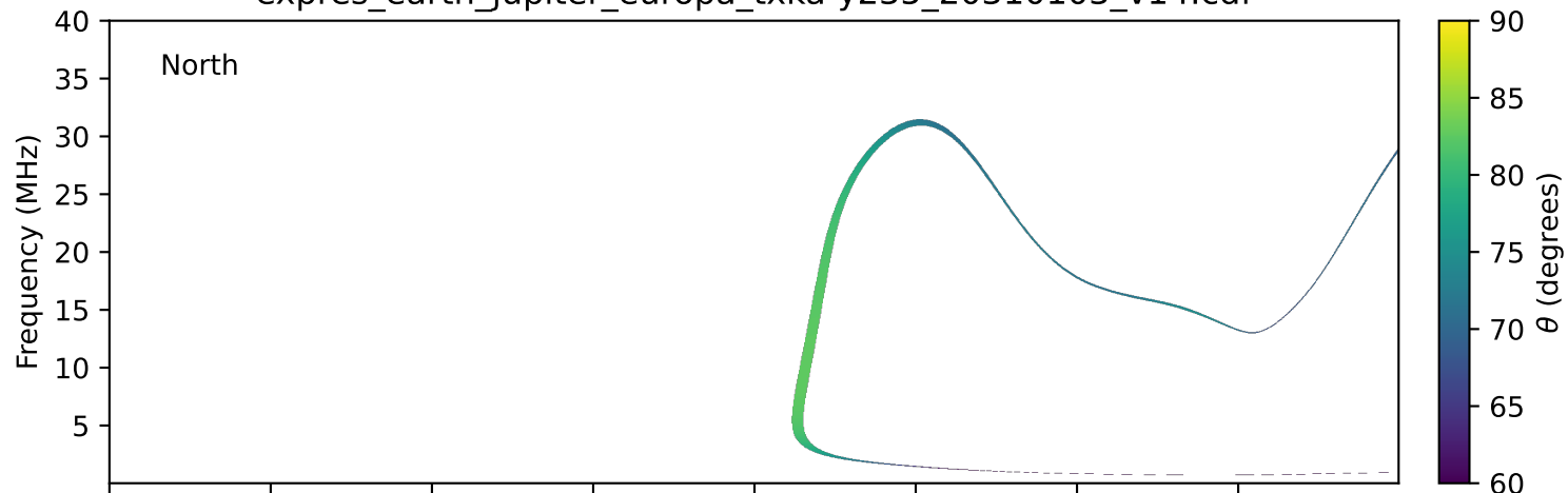
expres_earth_jupiter_europa_txka-y235_20310103_v14.cdf
