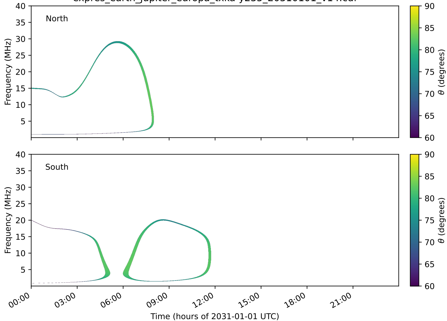
expres_earth_jupiter_europa_txka-y235_20310101_v14.cdf
