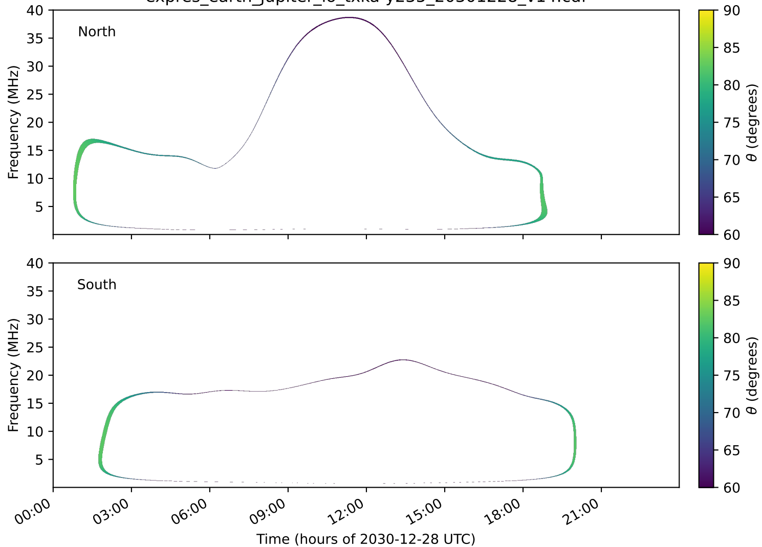
expres_earth_jupiter_io_txka-y235_20301228_v14.cdf
