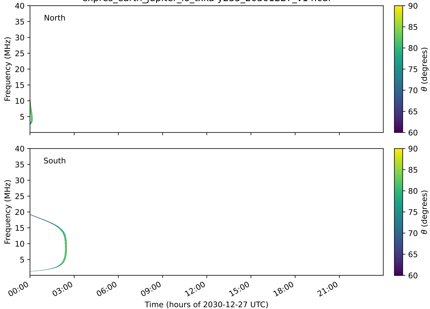
expres_earth_jupiter_io_txka-y235_20301227_v14.cdf
