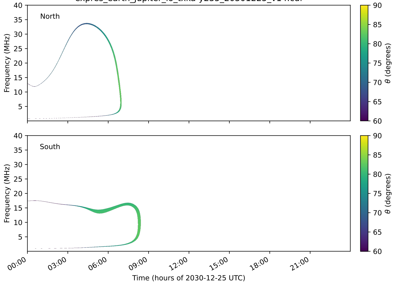
expres_earth_jupiter_io_txka-y235_20301225_v14.cdf
