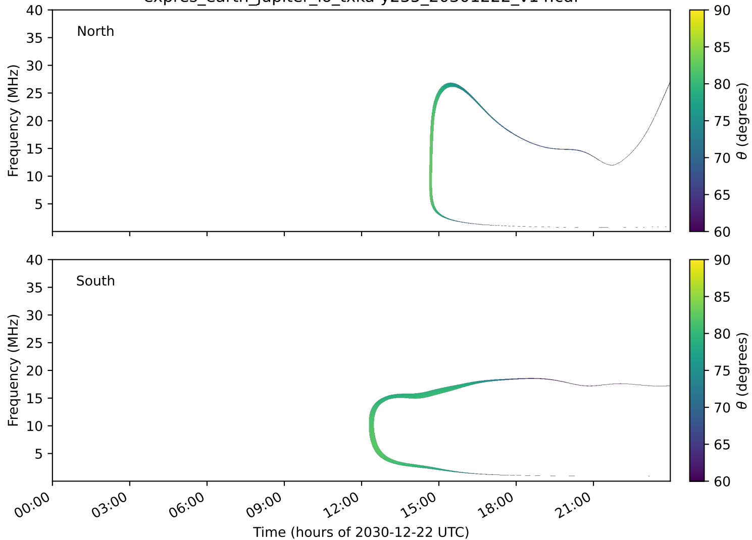
expres_earth_jupiter_io_txka-y235_20301222_v14.cdf
