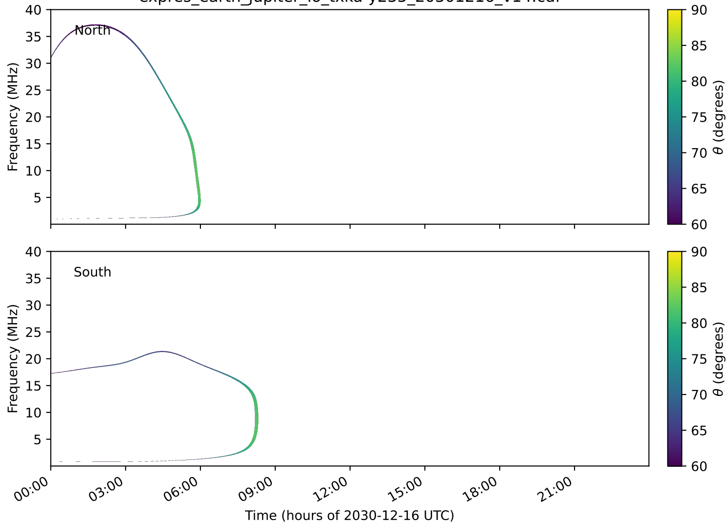
expres_earth_jupiter_io_txka-y235_20301216_v14.cdf
