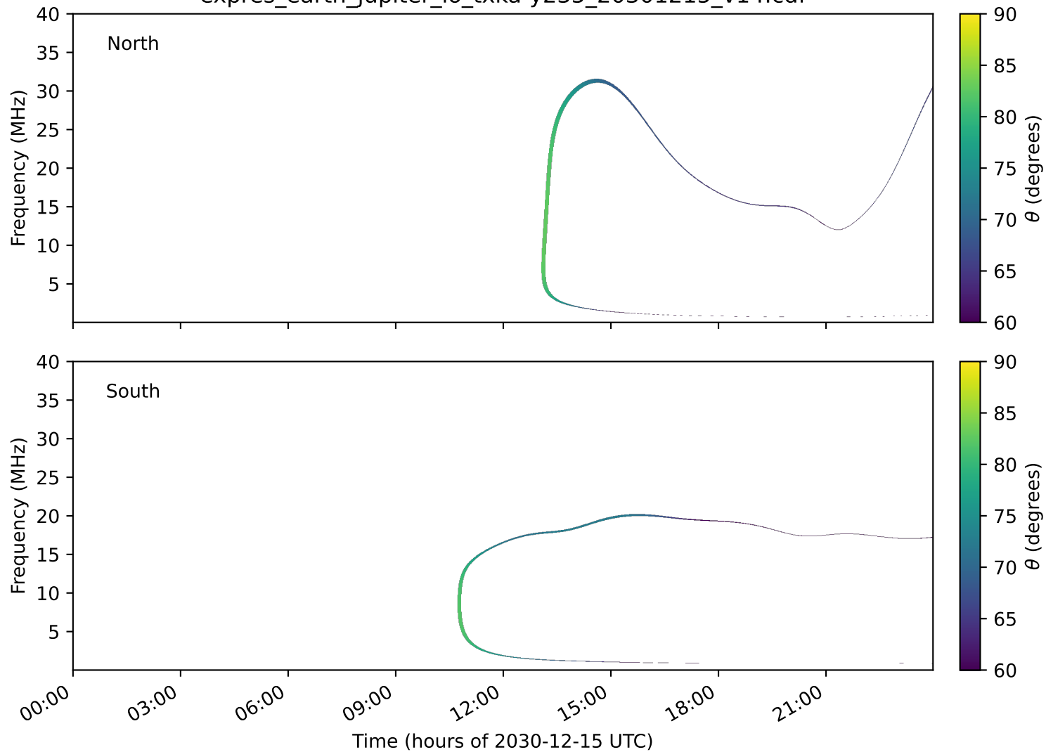
expres_earth_jupiter_io_txka-y235_20301215_v14.cdf
