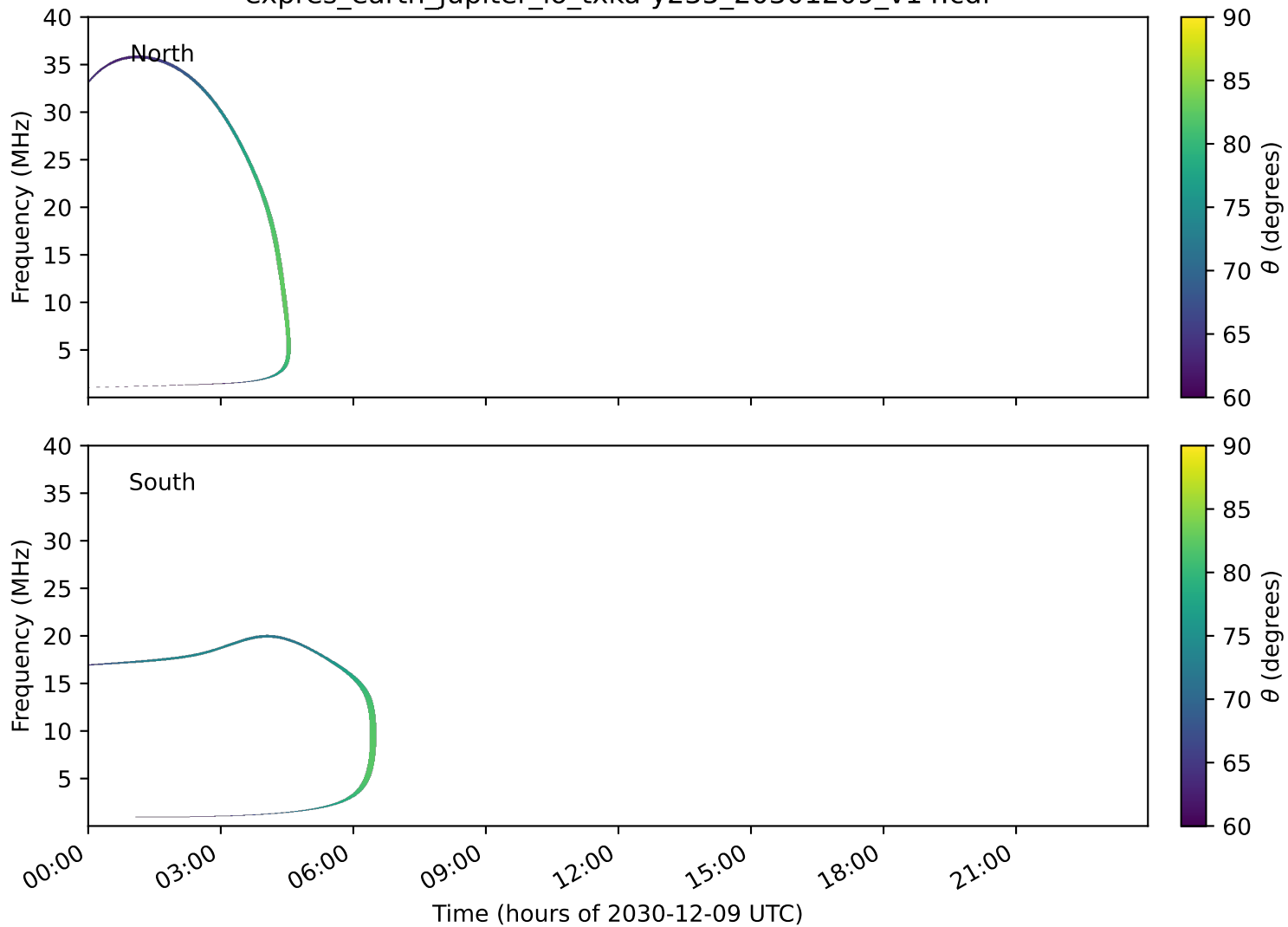
expres_earth_jupiter_io_txka-y235_20301209_v14.cdf
