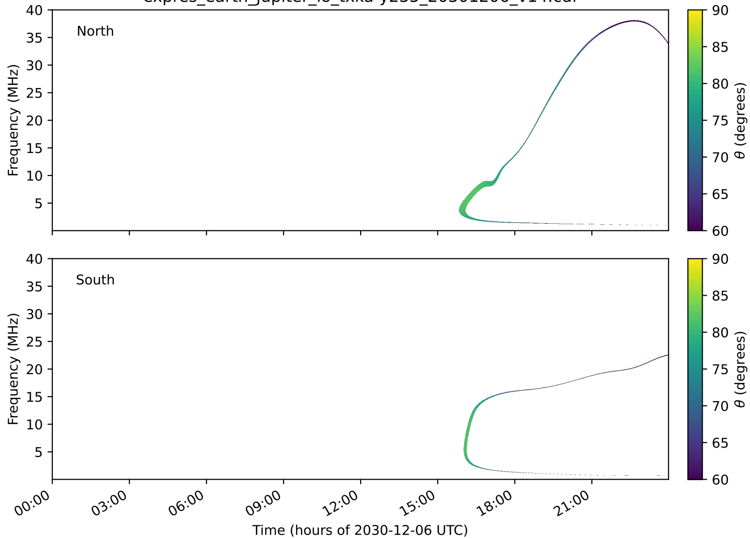
expres_earth_jupiter_io_txka-y235_20301206_v14.cdf
