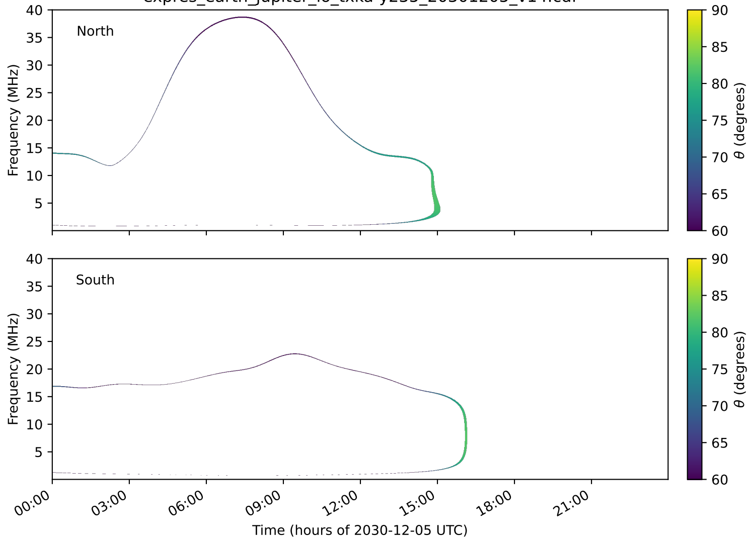
expres_earth_jupiter_io_txka-y235_20301205_v14.cdf
