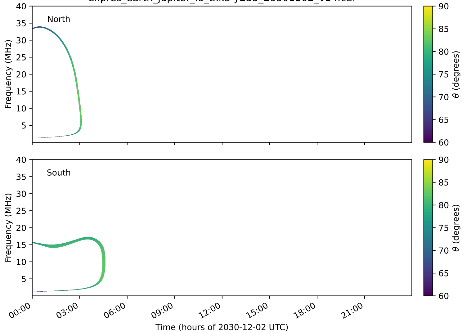
expres_earth_jupiter_io_txka-y235_20301202_v14.cdf
