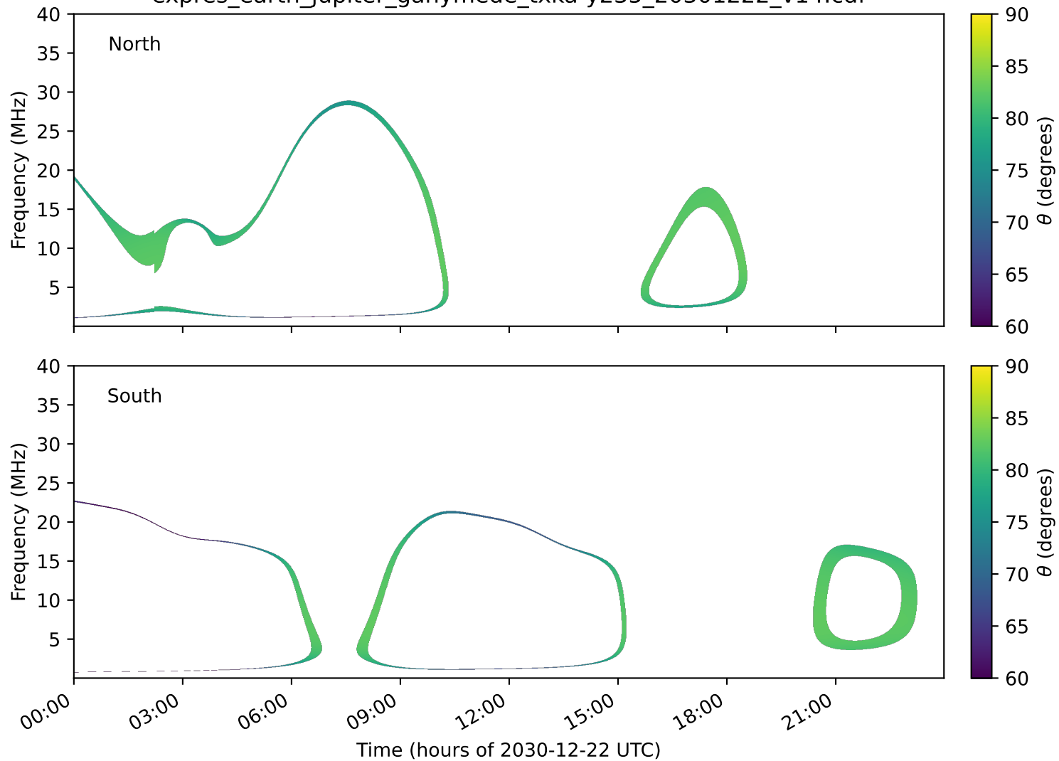
expres_earth_jupiter_ganymede_txka-y235_20301222_v14.cdf
