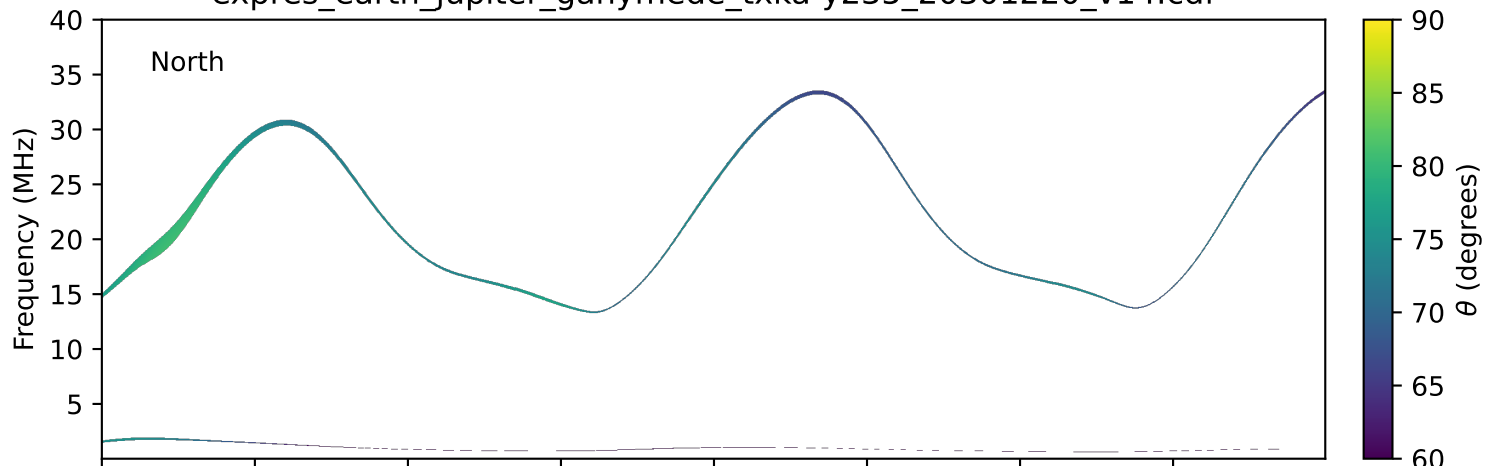
expres_earth_jupiter_ganymede_txka-y235_20301220_v14.cdf
