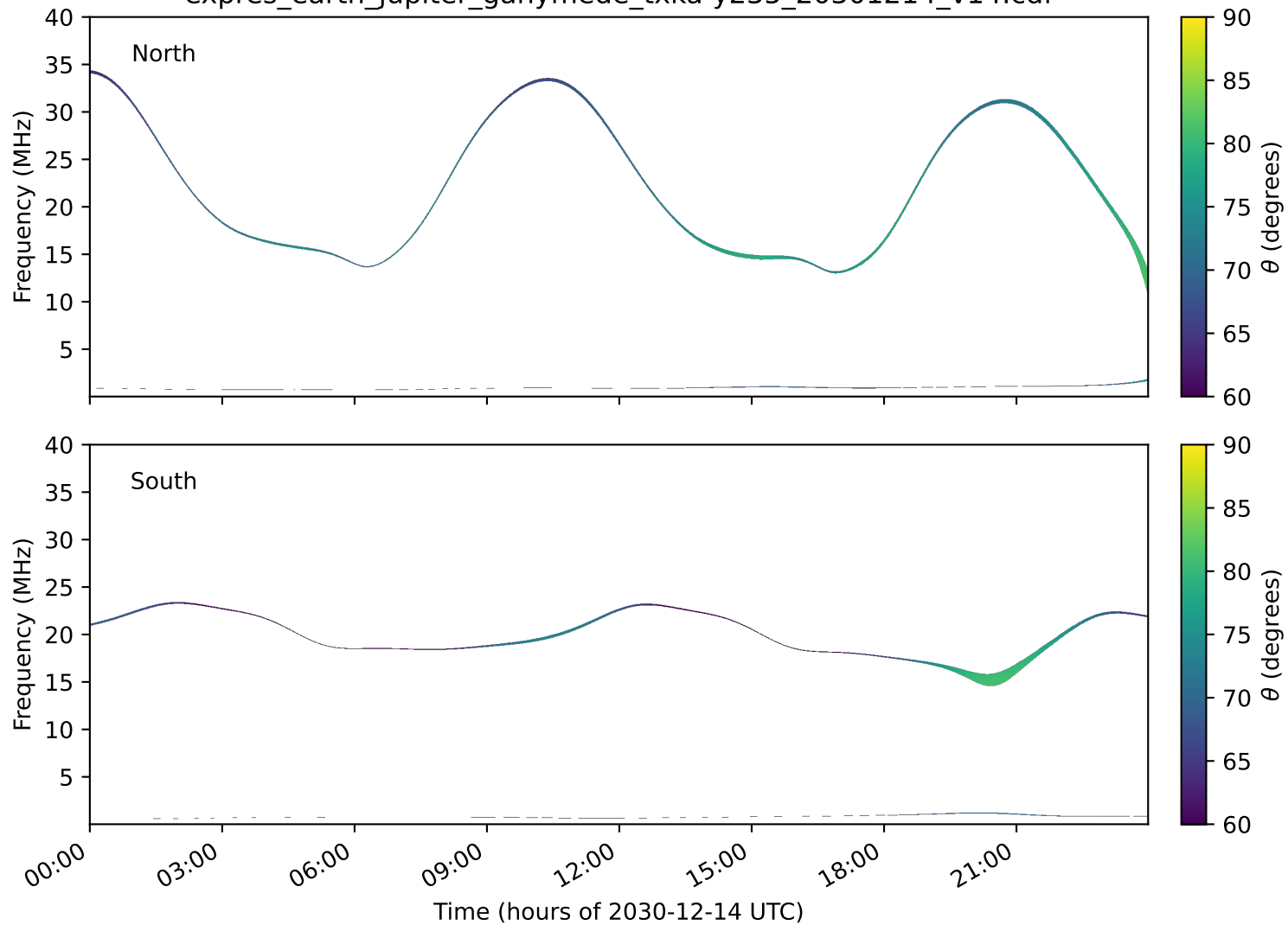
expres_earth_jupiter_ganymede_txka-y235_20301214_v14.cdf
