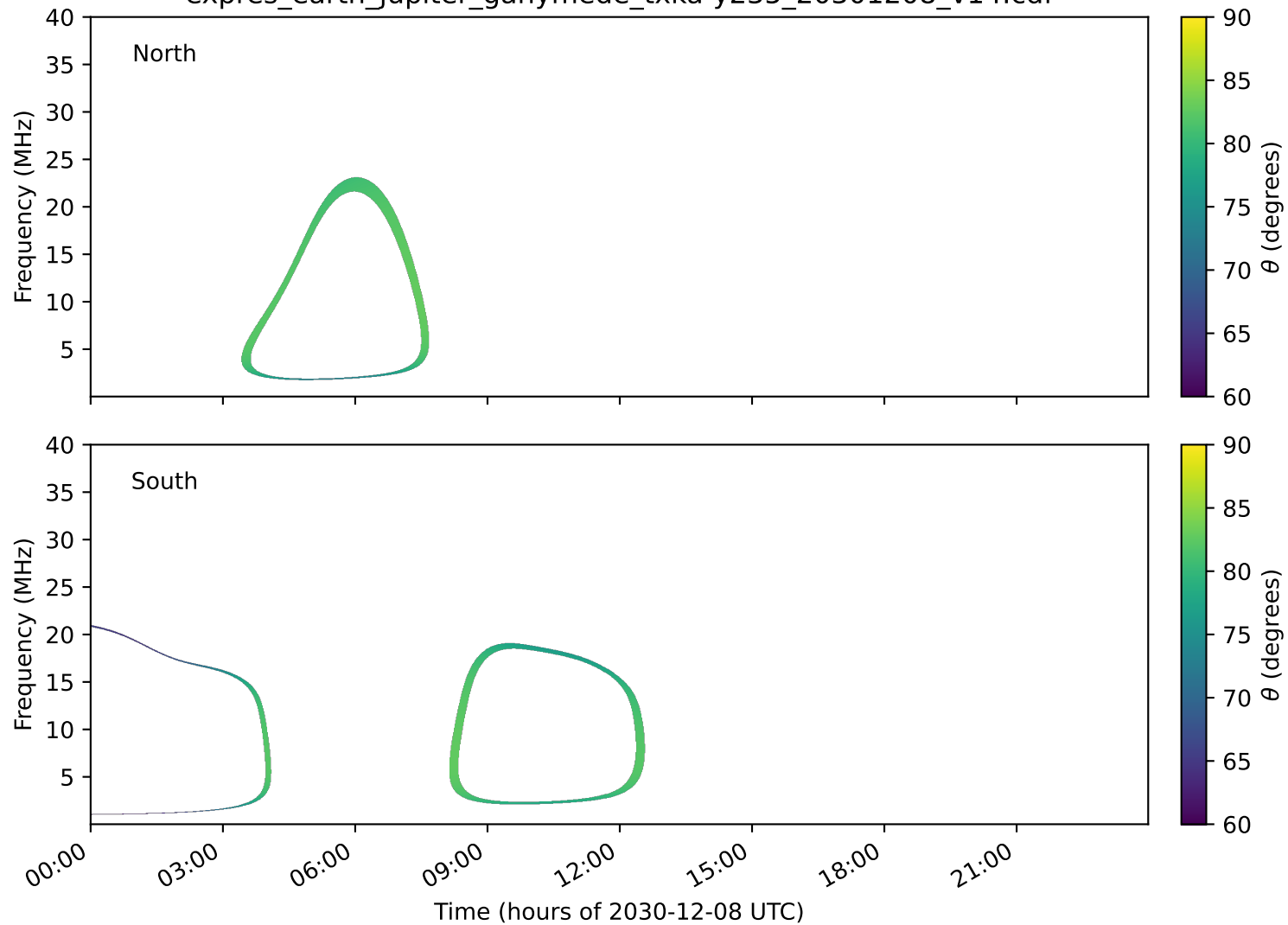
expres_earth_jupiter_ganymede_txka-y235_20301208_v14.cdf
