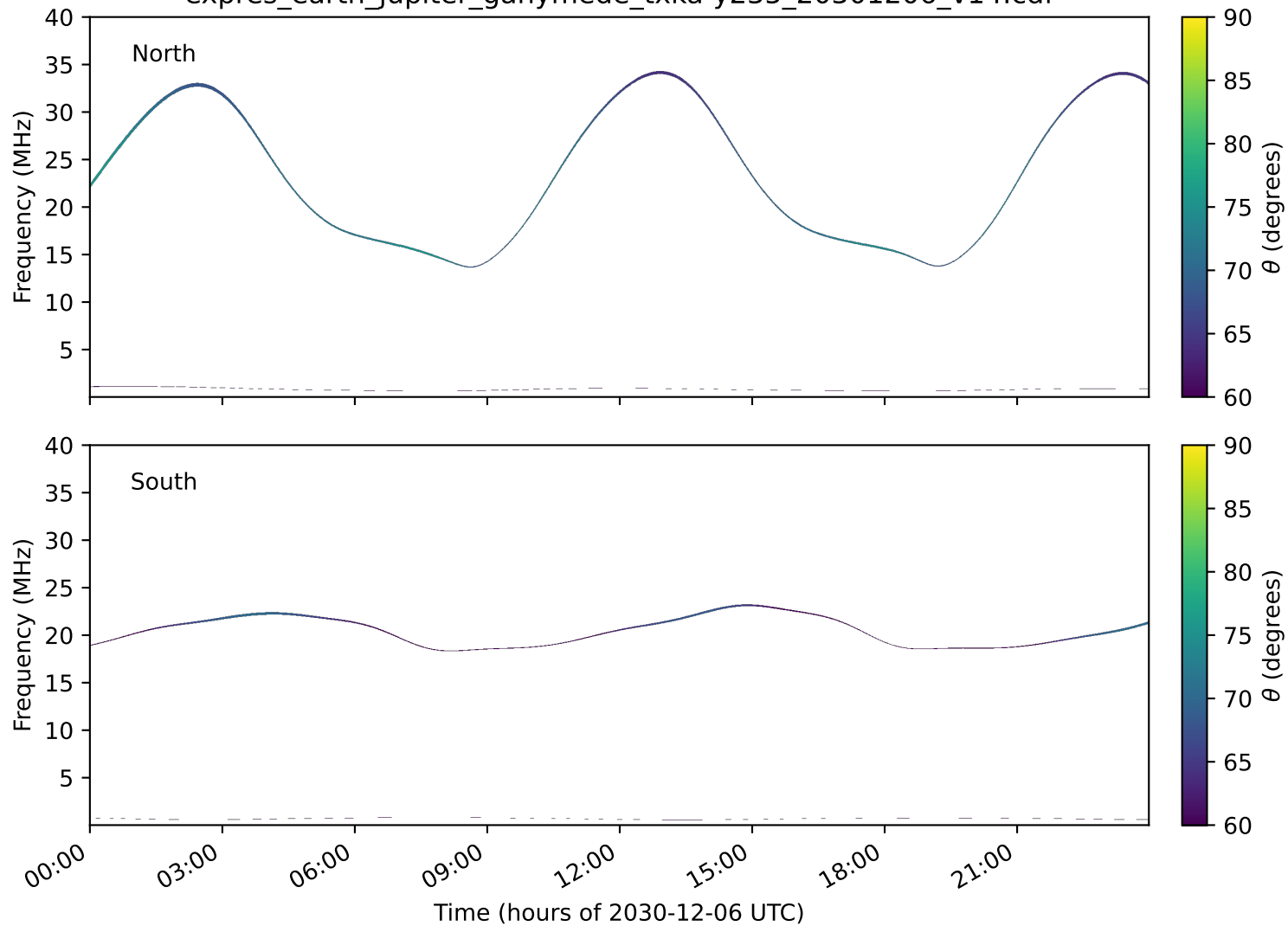
expres_earth_jupiter_ganymede_txka-y235_20301206_v14.cdf
