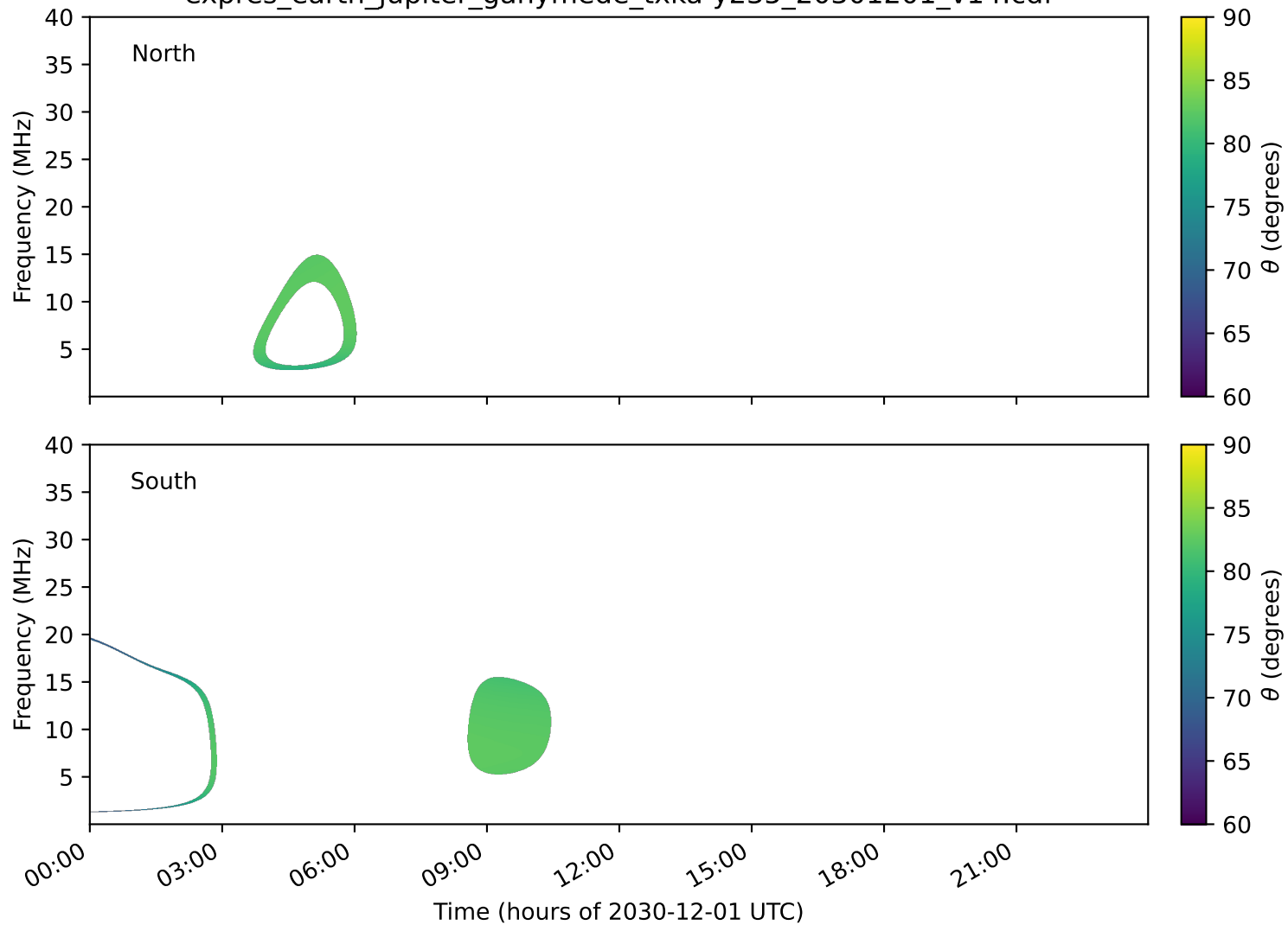
expres_earth_jupiter_ganymede_txka-y235_20301201_v14.cdf
