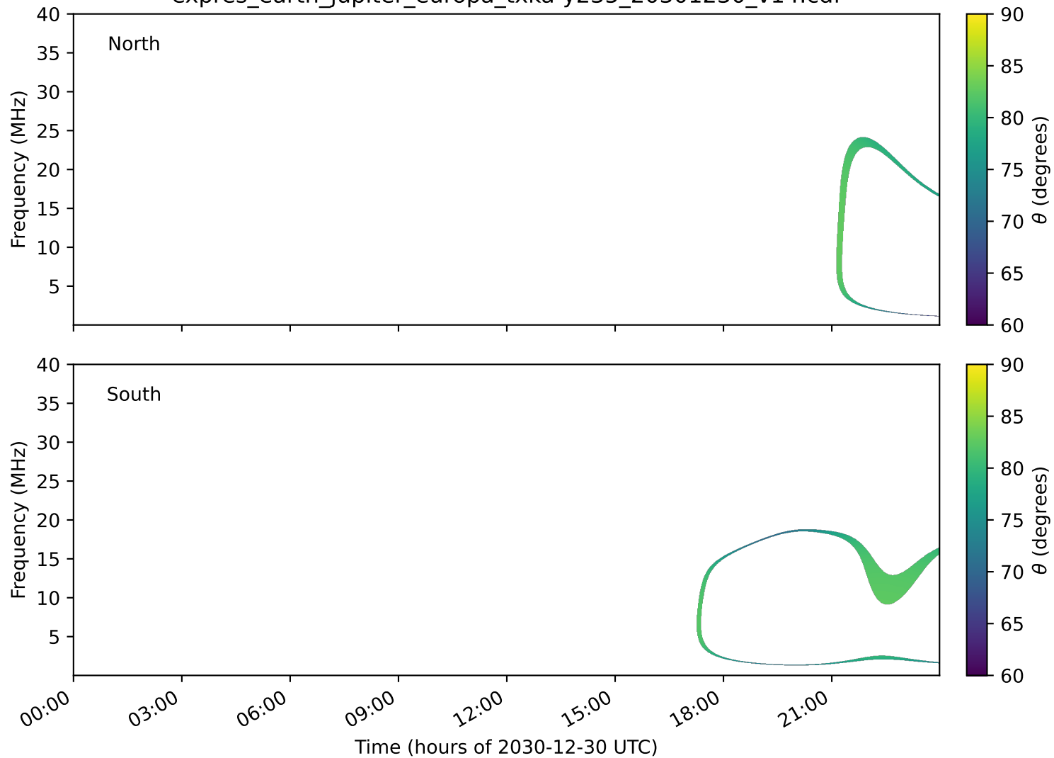
expres_earth_jupiter_europa_txka-y235_20301230_v14.cdf
