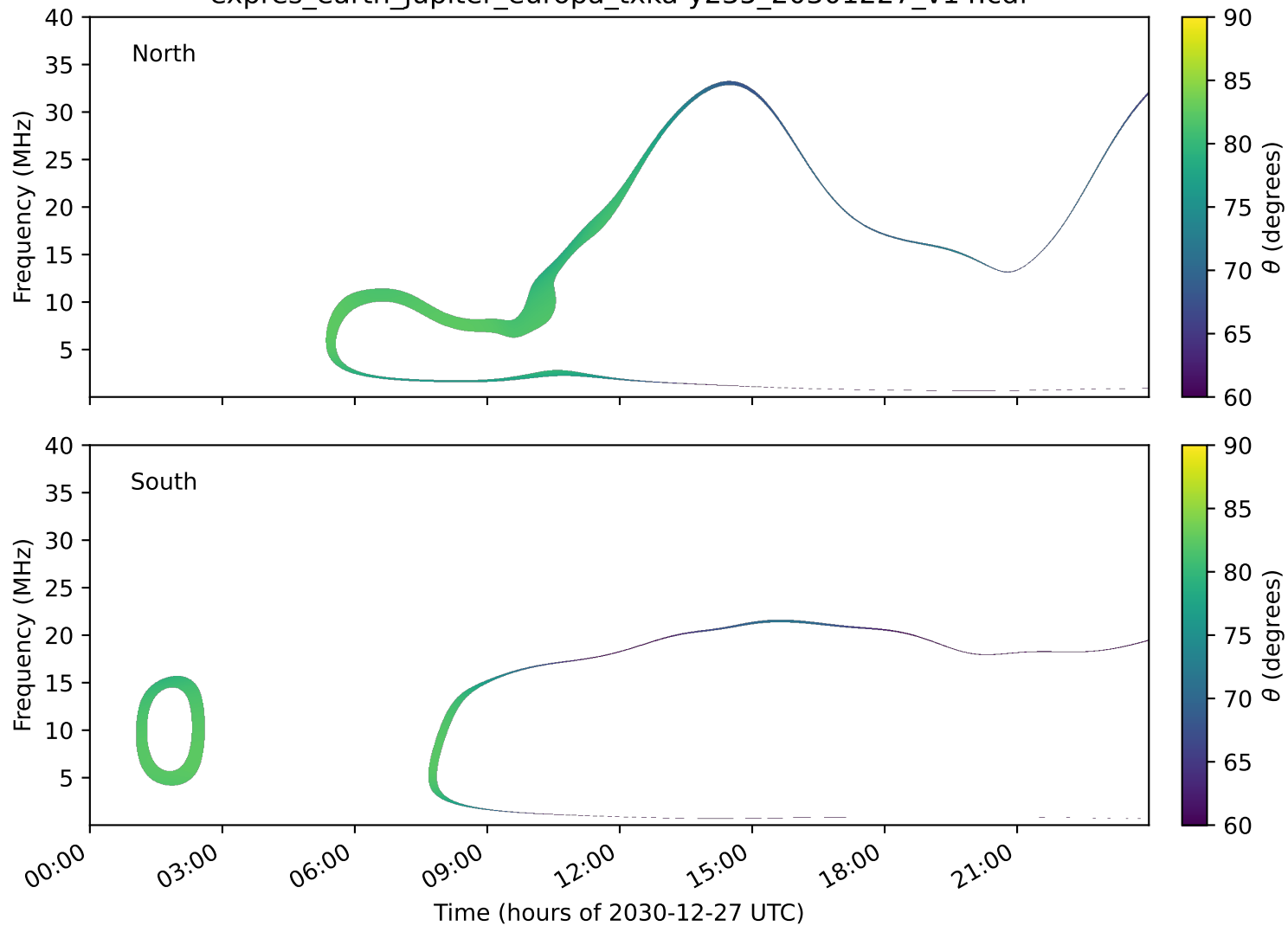
expres_earth_jupiter_europa_txka-y235_20301227_v14.cdf
