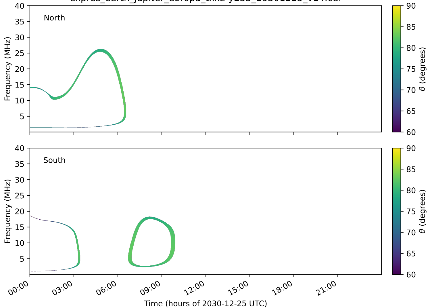
expres_earth_jupiter_europa_txka-y235_20301225_v14.cdf
