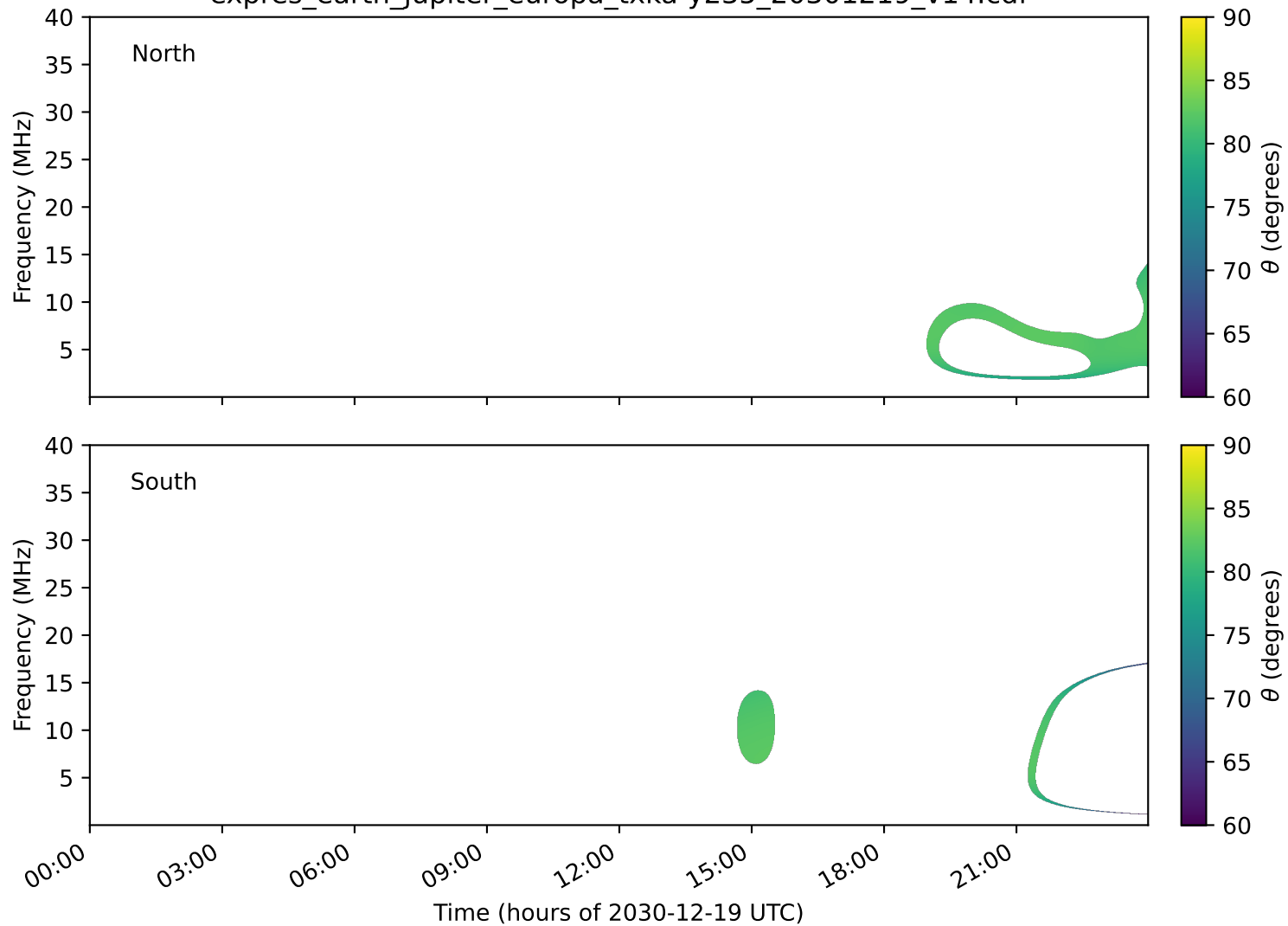
expres_earth_jupiter_europa_txka-y235_20301219_v14.cdf
