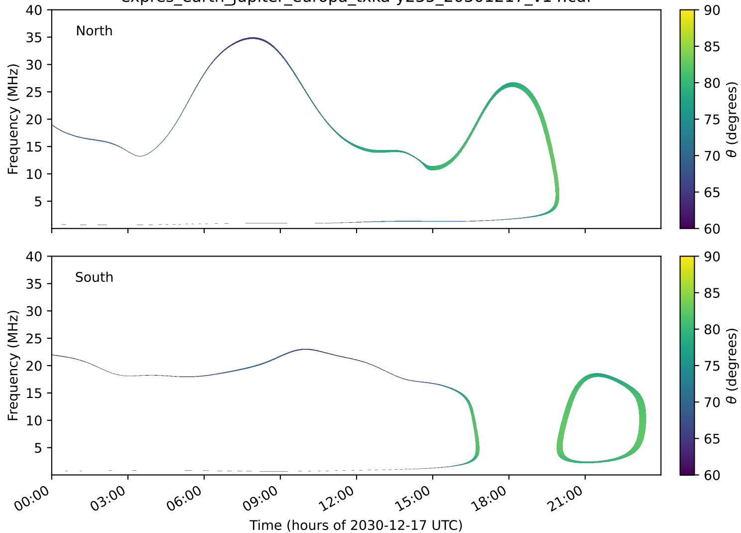
expres_earth_jupiter_europa_txka-y235_20301217_v14.cdf
