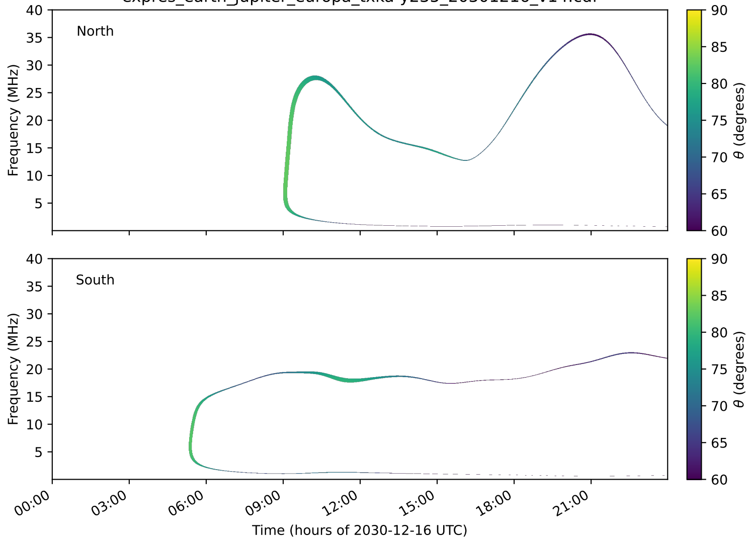
expres_earth_jupiter_europa_txka-y235_20301216_v14.cdf
