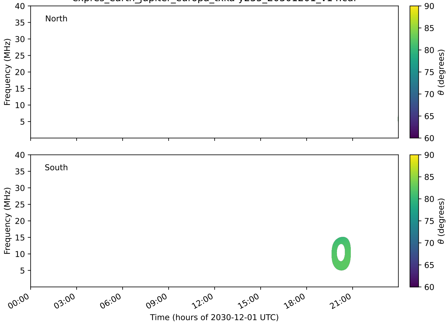
expres_earth_jupiter_europa_txka-y235_20301201_v14.cdf
