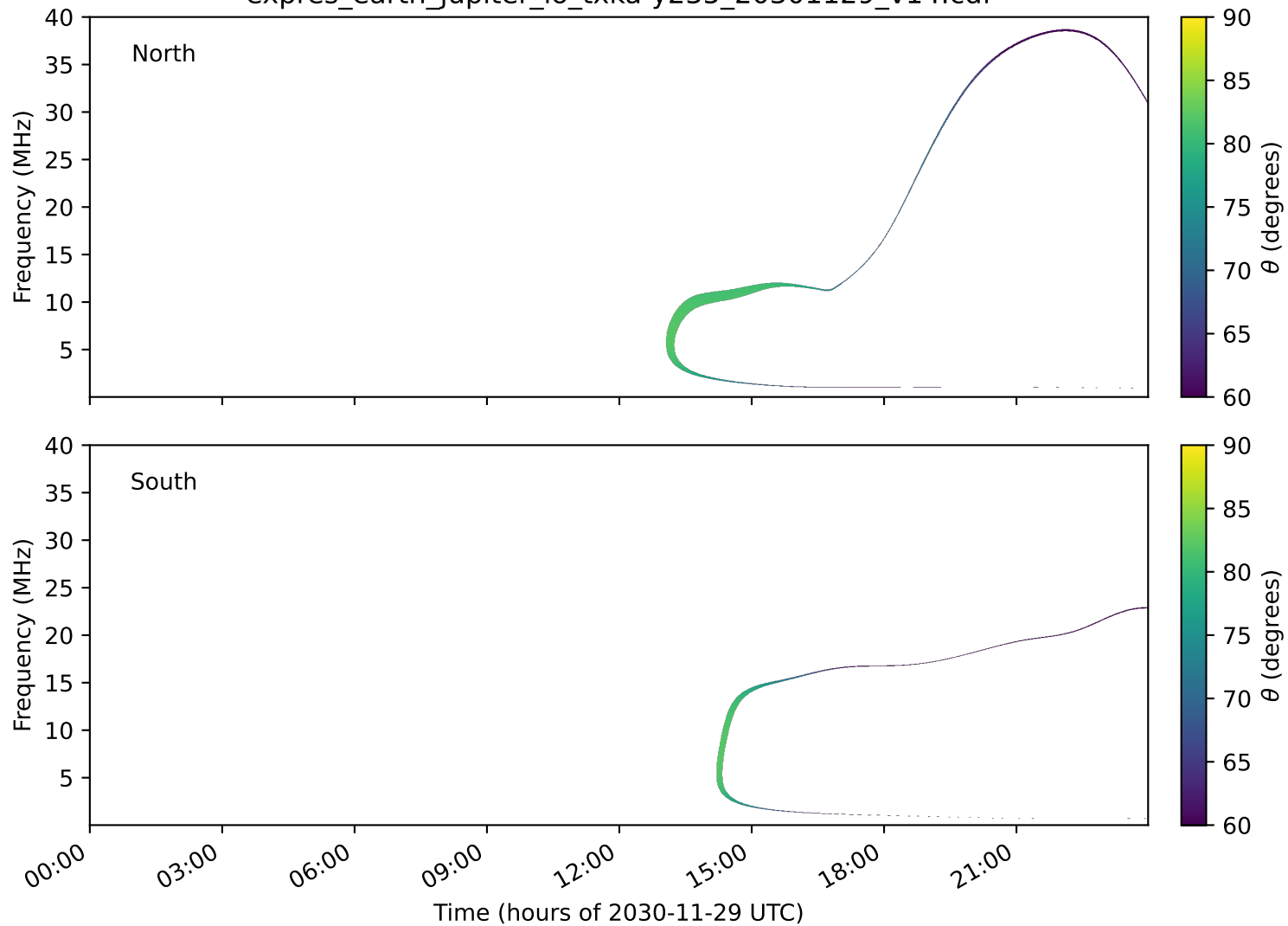
expres_earth_jupiter_io_txka-y235_20301129_v14.cdf
