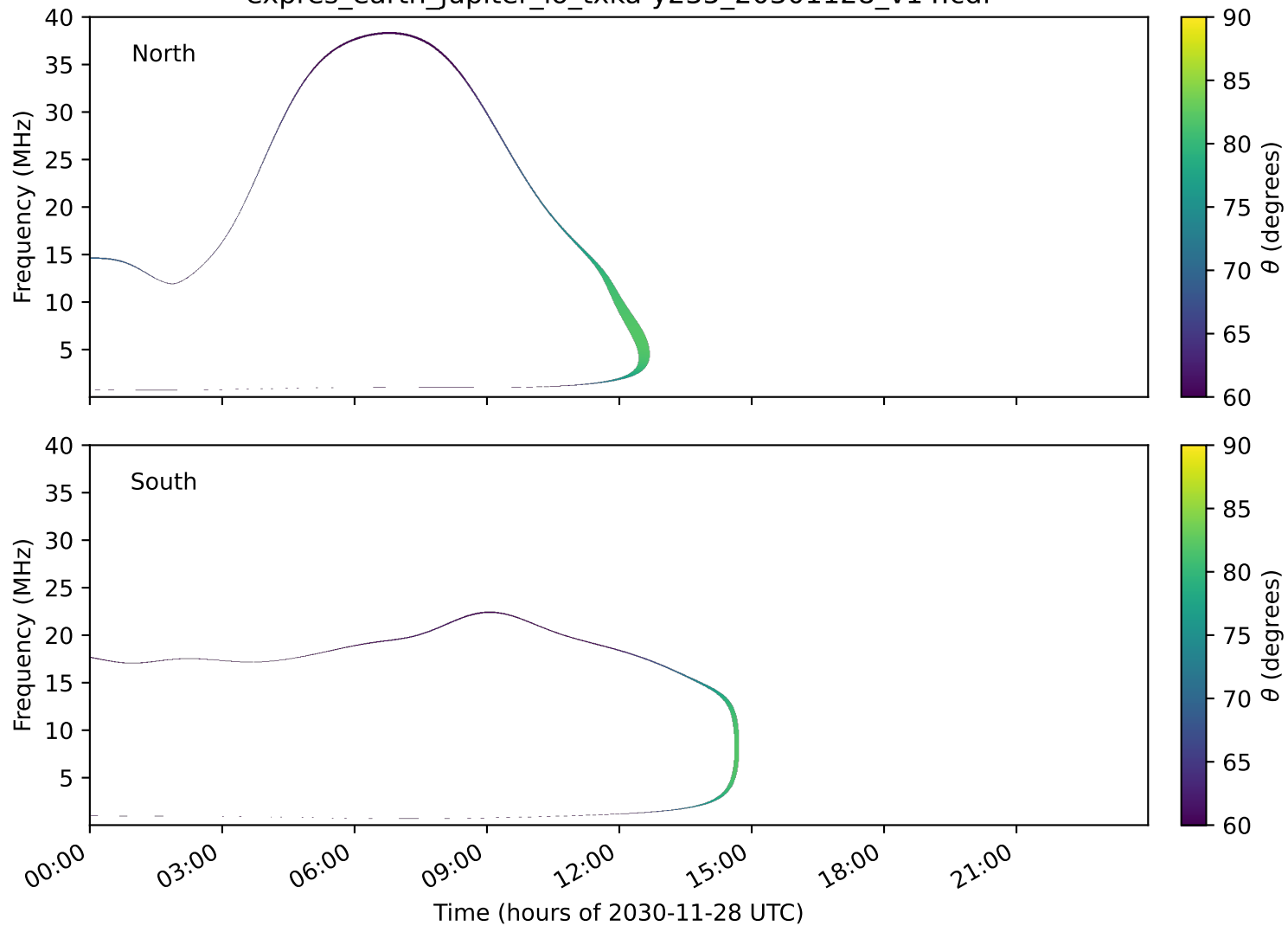
expres_earth_jupiter_io_txka-y235_20301128_v14.cdf
