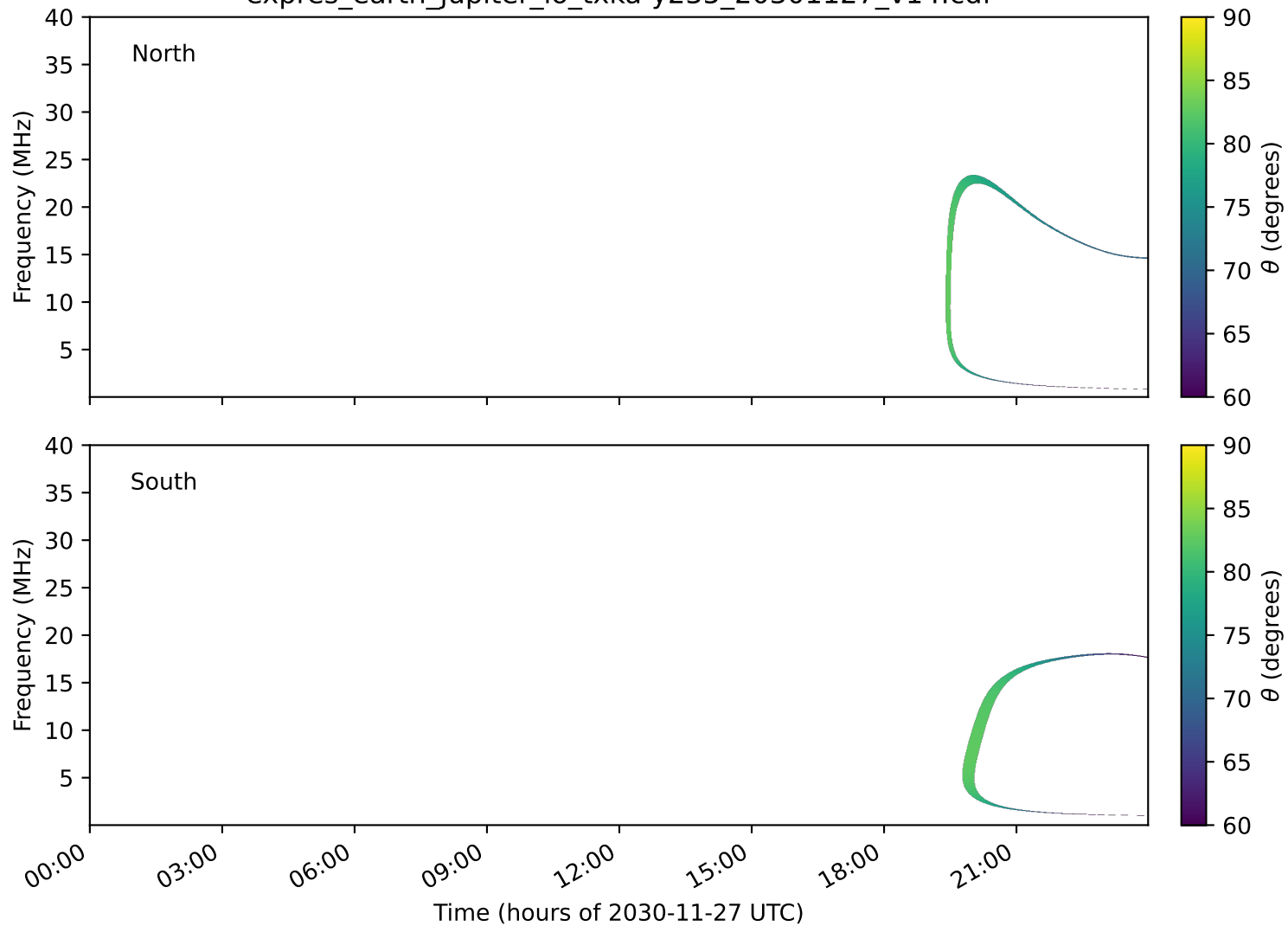
expres_earth_jupiter_io_txka-y235_20301127_v14.cdf
