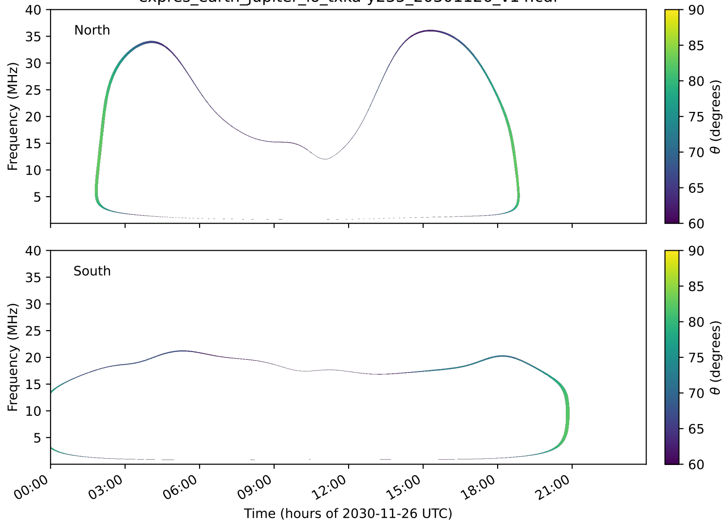
expres_earth_jupiter_io_txka-y235_20301126_v14.cdf
